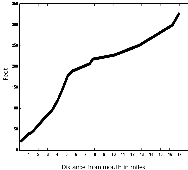
Figure 3. Elevation of watershed by river mile
